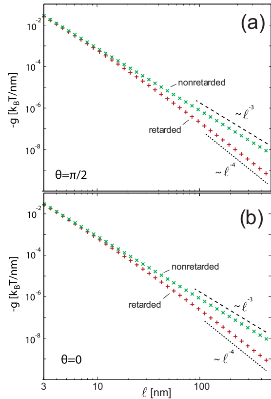
FIG. 3. (Color online) vdW interaction for a (6,5) carbon nanotube above a half space made of (6,5) carbon nanotubes as a function of distance ( \epsilon_3=1 ) for \theta=\pi/2 (panel a) and \theta=0 (panel b). The values of dispersion interaction with retardation included are indicated by (red) pluses. The nonretarded values are indicated by (green) \times 's. The power-law behaviors l^{-4} and l^{-3} are denoted by dotted and dashed lines, respectively.
